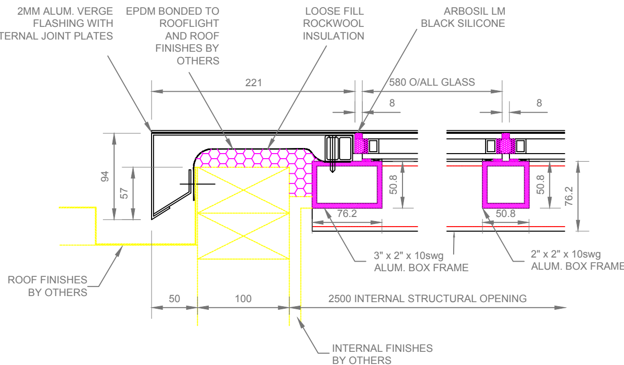
SECTION C-C
