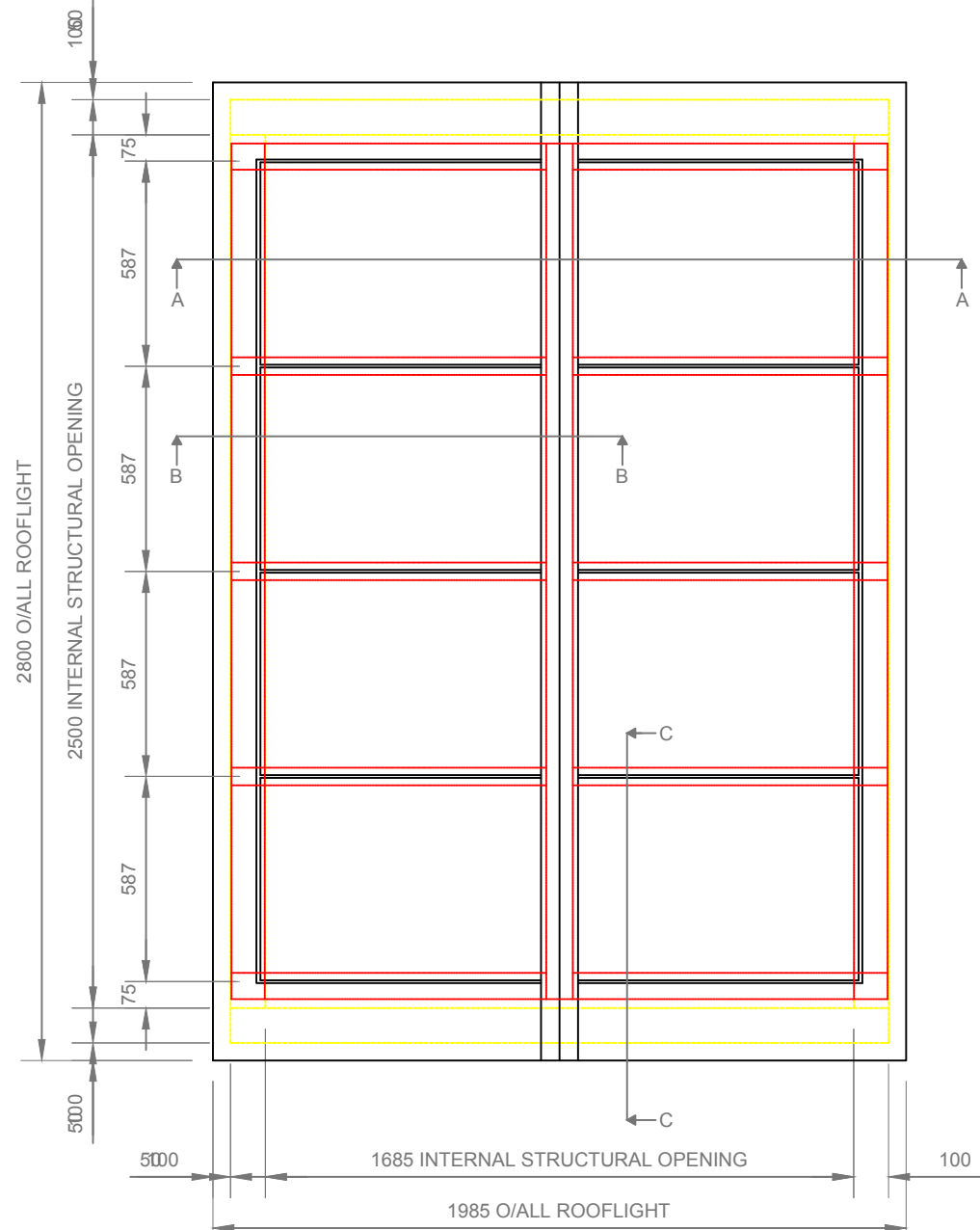
PLAN
