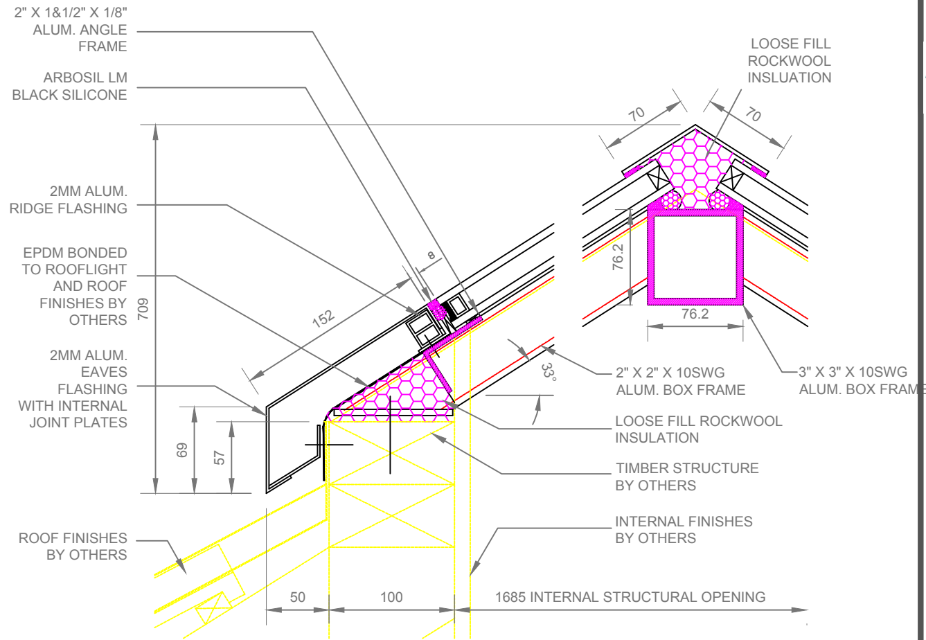
SECTION B-B
