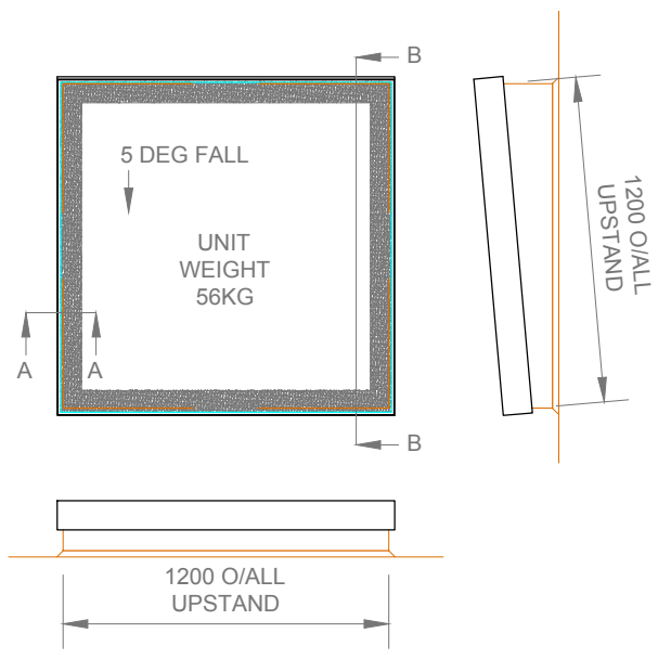
PLAN AND ELEVATIONS SCALE 1:30 (A3)
