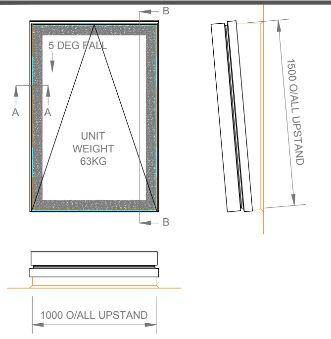
PLAN AND ELEVATIONS SCALE NTS(A3)
