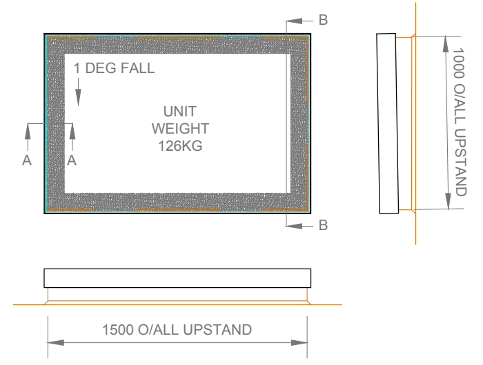
PLAN AND ELEVATIONS SCALE 1:30 (A3)
